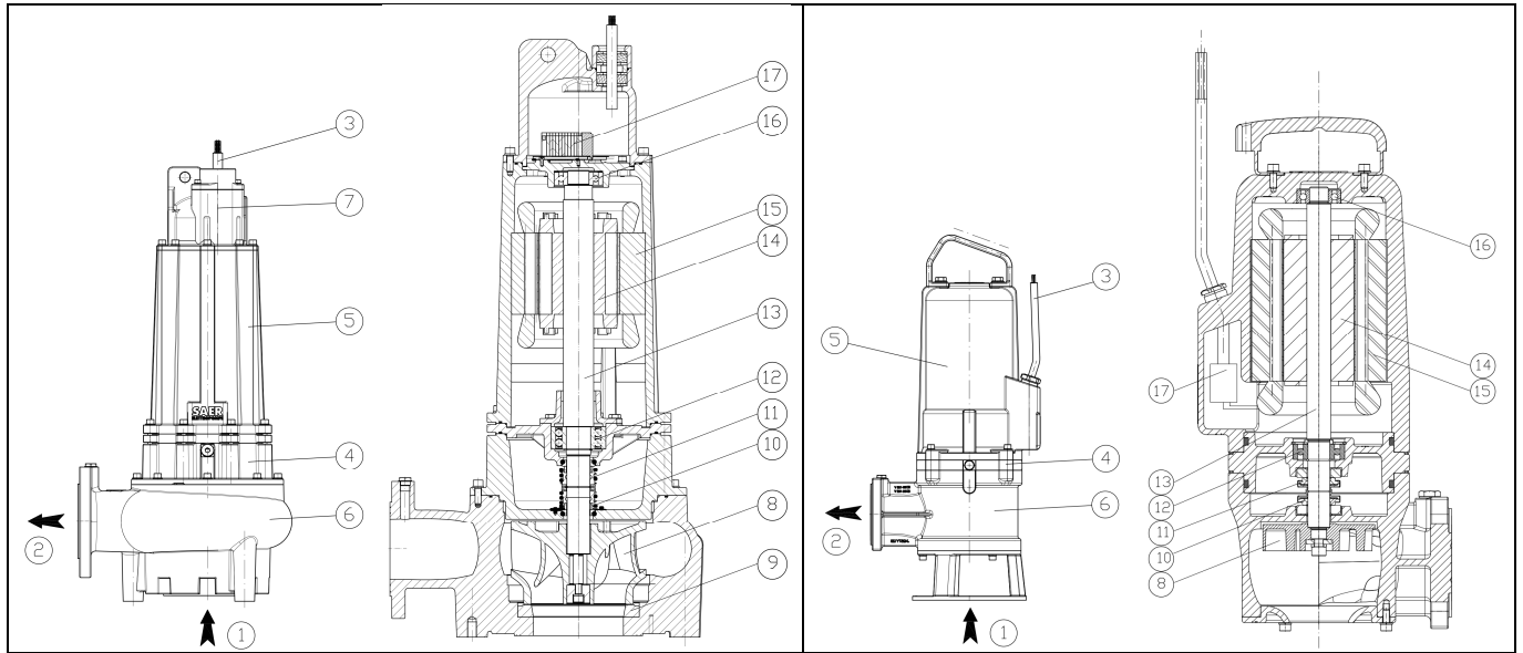
FIG. 2 COMPONENTI PRINCIPALI • MAIN COMPONENTS
