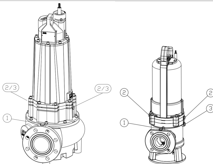
FIG. 6 TAPPI E CONNESSIONI AUSILIARIE • PLUGS AND AUXILIARY CONNECTIONS
